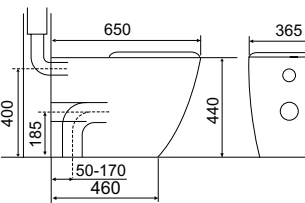
ELLISSE OVERHEIGHT MK II TOILET PAN
