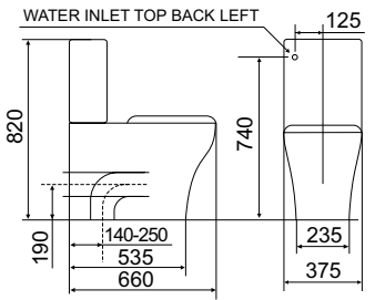
CYGNET OVERHEIGHT TOILET SUITE
