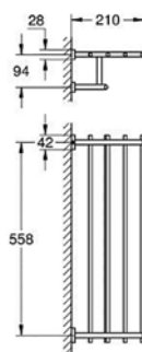
40 512 001 Multi-towel rack 558mm
