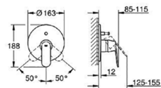
19 382 000 + 33 961 000 Shower/bath mixer with diverter
