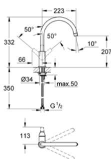
31 230 000 BauFlow Kitchen sink mixer
