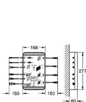
36 397 000 Base unit box 2.0 Bluetooth 26 374 000 Base unit box 4.0 Bluetooth
