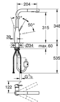
30 270 000 / 30 270 DC0 Sink mixer high spout with Pull-Out Dual Spray
