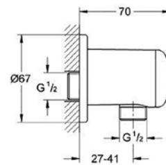
28 671 000 Relexa Shower outlet elbow 1/2"
