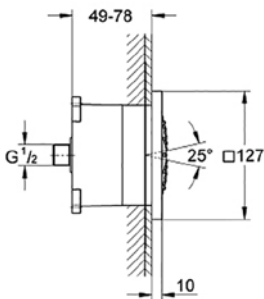
27 251 000 Rainshower® F-Series 5" 127 x 127mm
