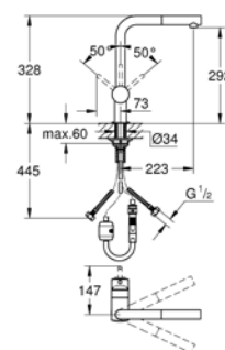
31 115 000 Sink mixer L-spout with Pull-Out Spray
