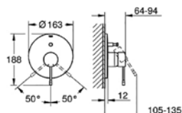
19 285 001 + 33 961 000 Shower/bath mixer with diverter
