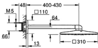
26 479 000 Rainshower 310 Head shower with wall arm
