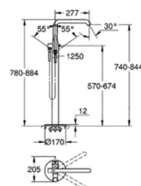
23 491 001 + 45 984 001 Floormounted bath/shower mixer
