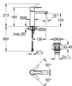
23 106 001 Basin mixer with Push-up open waste set
