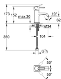
32 759 000 M-Size Basin mixer
